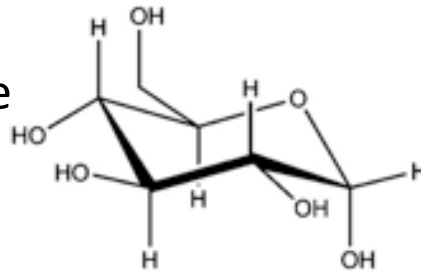
Glucose (α-pyranose form)
