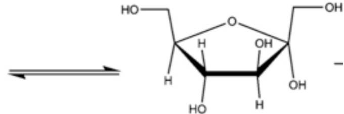
Fructose (α-furanose form)
