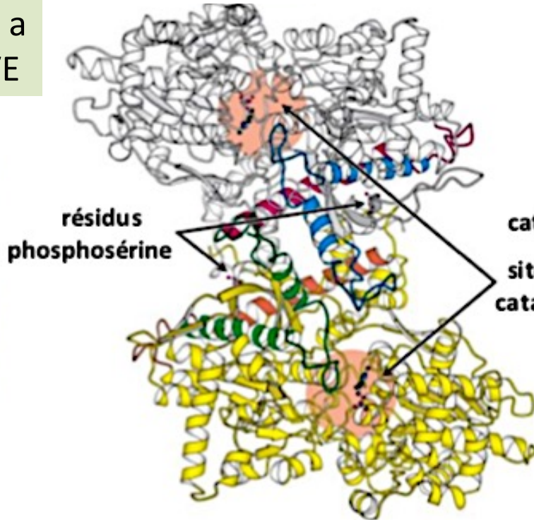
Phosphorylase a
